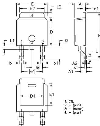
X004 TO-252 AA (D PAK)
