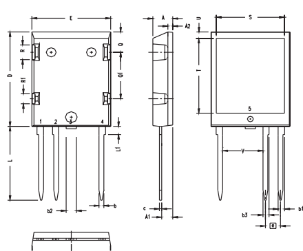
X022c ISOPLUS264 (3HV)
