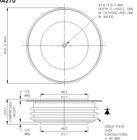
W6 - 100A270
