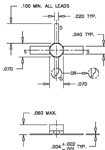
Package 73
