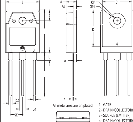
X017a TO-3P
