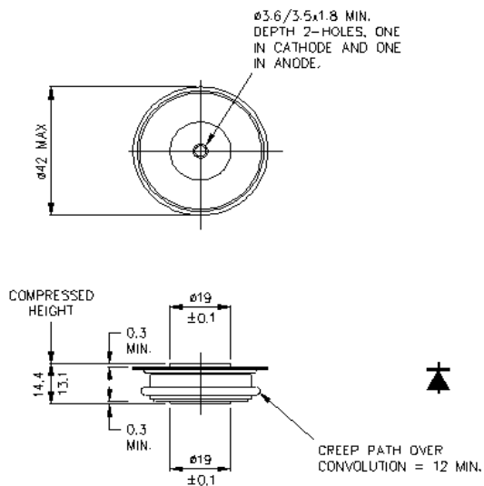
W1 - 100A241
