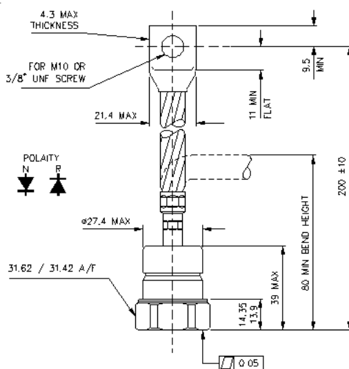
W26 - 100A283
