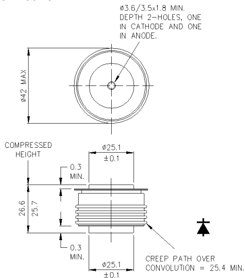
W5 - 100A249
