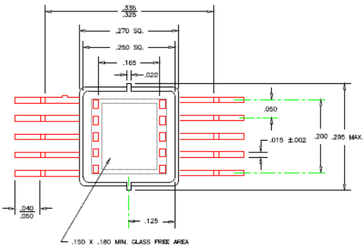
Package 99
