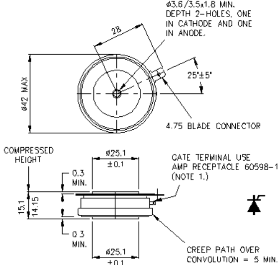
W9 - 101A335
