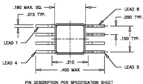
Package 87
