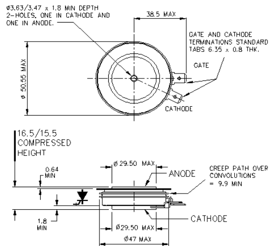
W34 - 101A287
