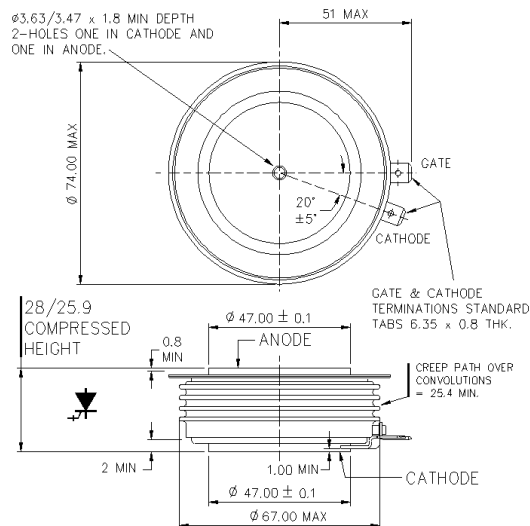
W36 - 101A288
