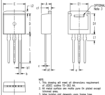
X008 TO-262 I 2 PAK
