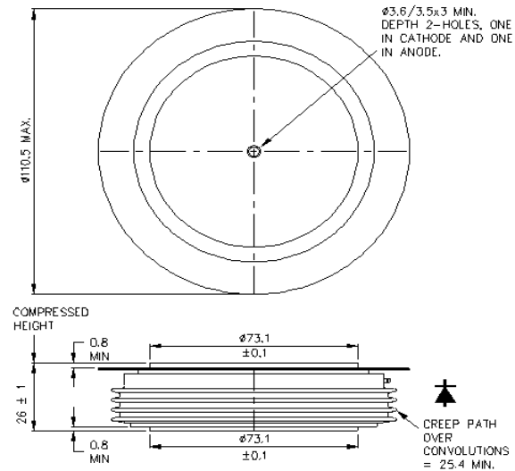
W42 - 100A310
