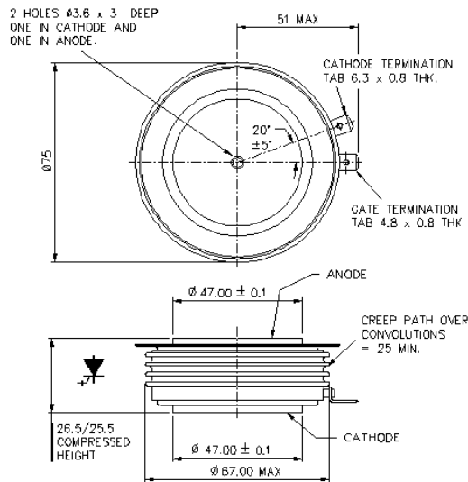
W30 - 101A343
