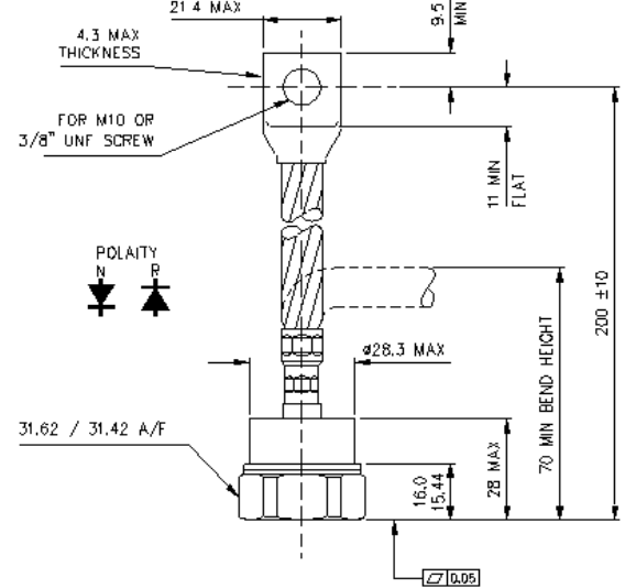
W27 - 100A284
