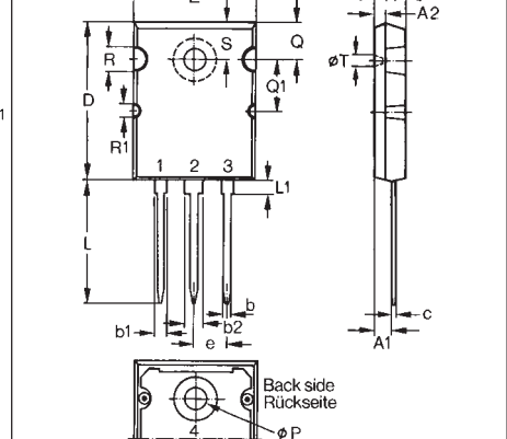
X020 TO-264 AA
