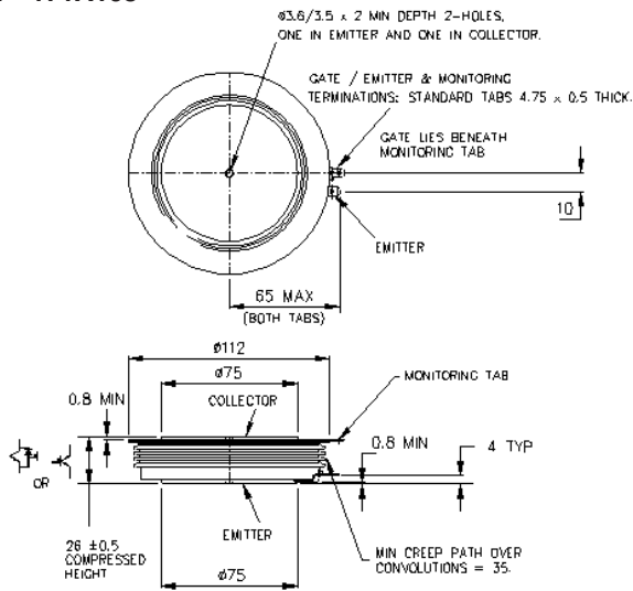
W41 - 171A108
