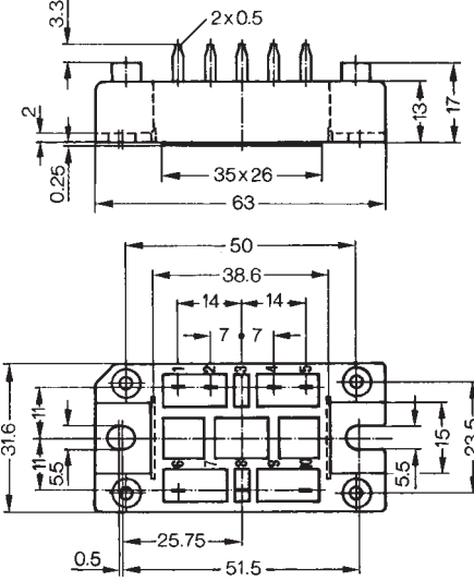
X103 V1-A-Pack
