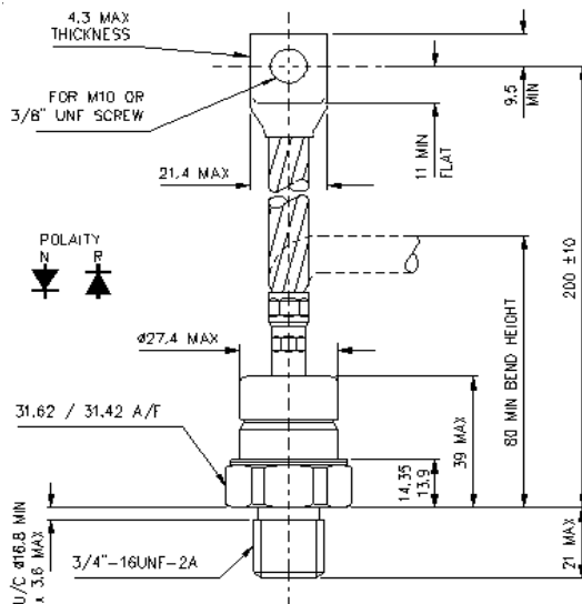
W24 - 100A280
