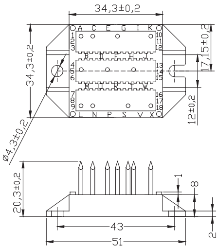
X102 ECO-PAC2
