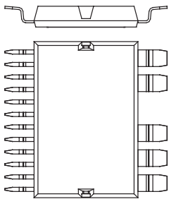
X026c ISOPLUS-DIL™ Weight = 25 g xxx-SMD
