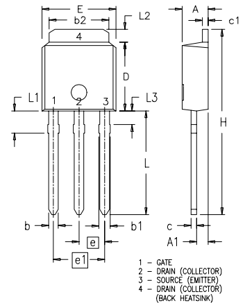
X003 TO-251 AA
