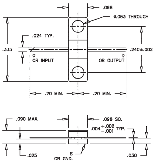
Package 71
