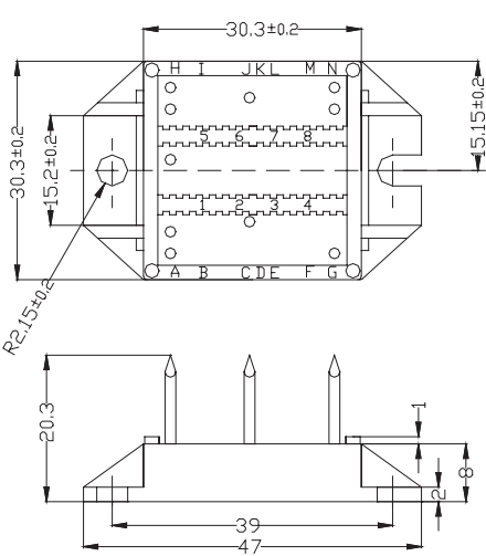
X101 ECO-PAC1
