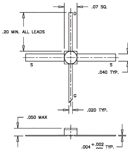
Package 73
